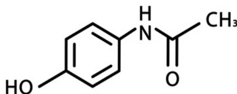
Paracetamol C 8 H 9 NO 2
